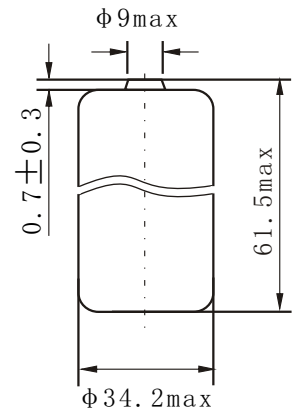
Dimensions in mm S/: STANDARD
