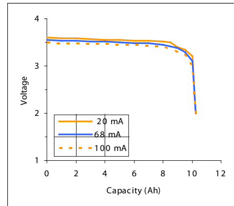
125°C discharge
